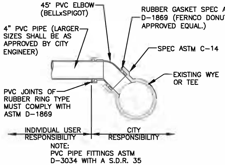
Connecting into Existing Wye or Tee
