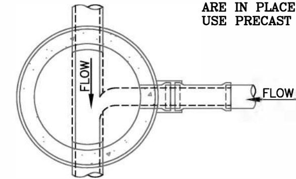
STANDARD MANHOLE PLAN VIEW
