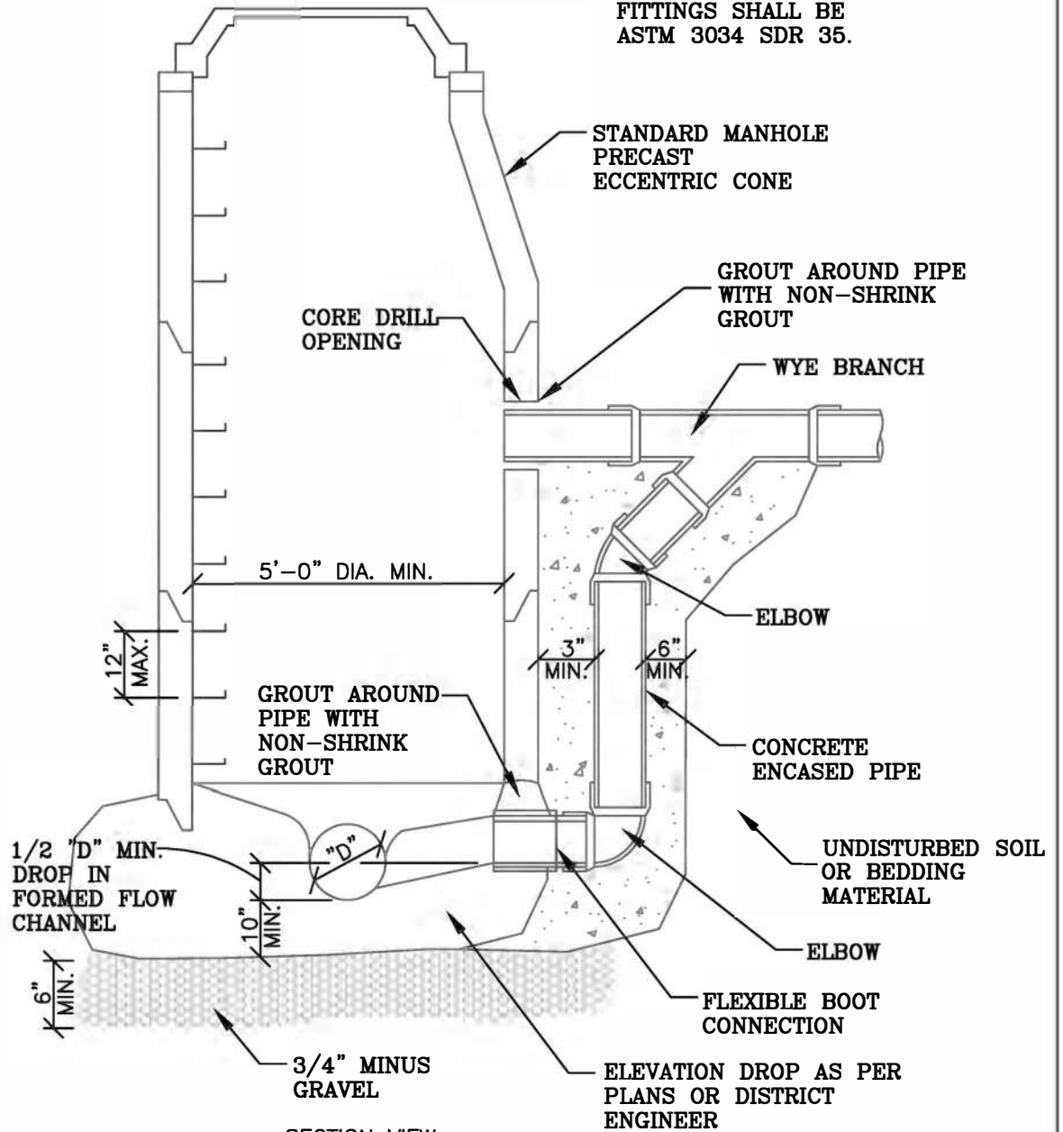
SECTION VIEW
