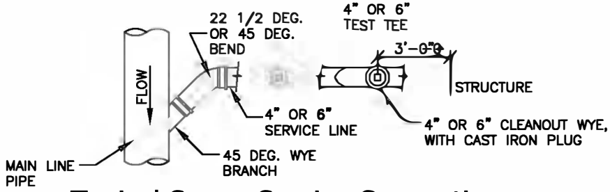
Typical Sewer Service Connection
