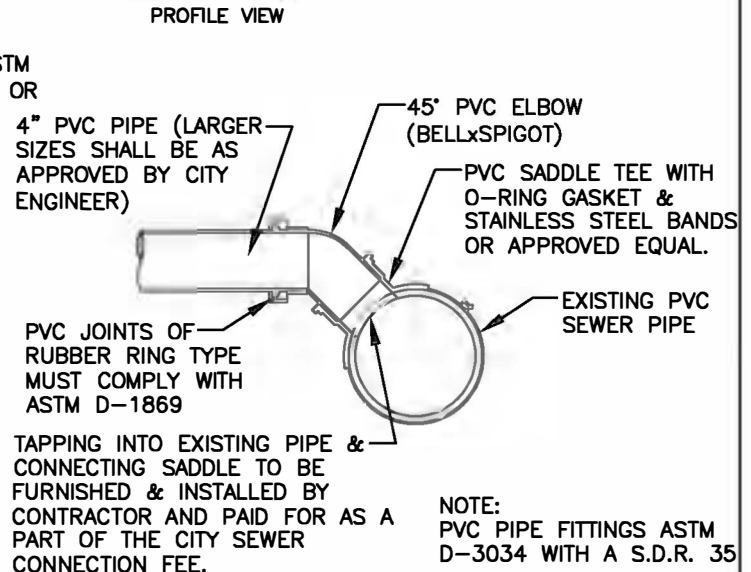
Tapping into Existing PVC Pipe
