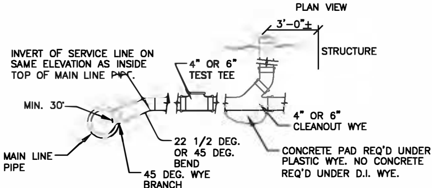
Typical Sewer Service Connection
